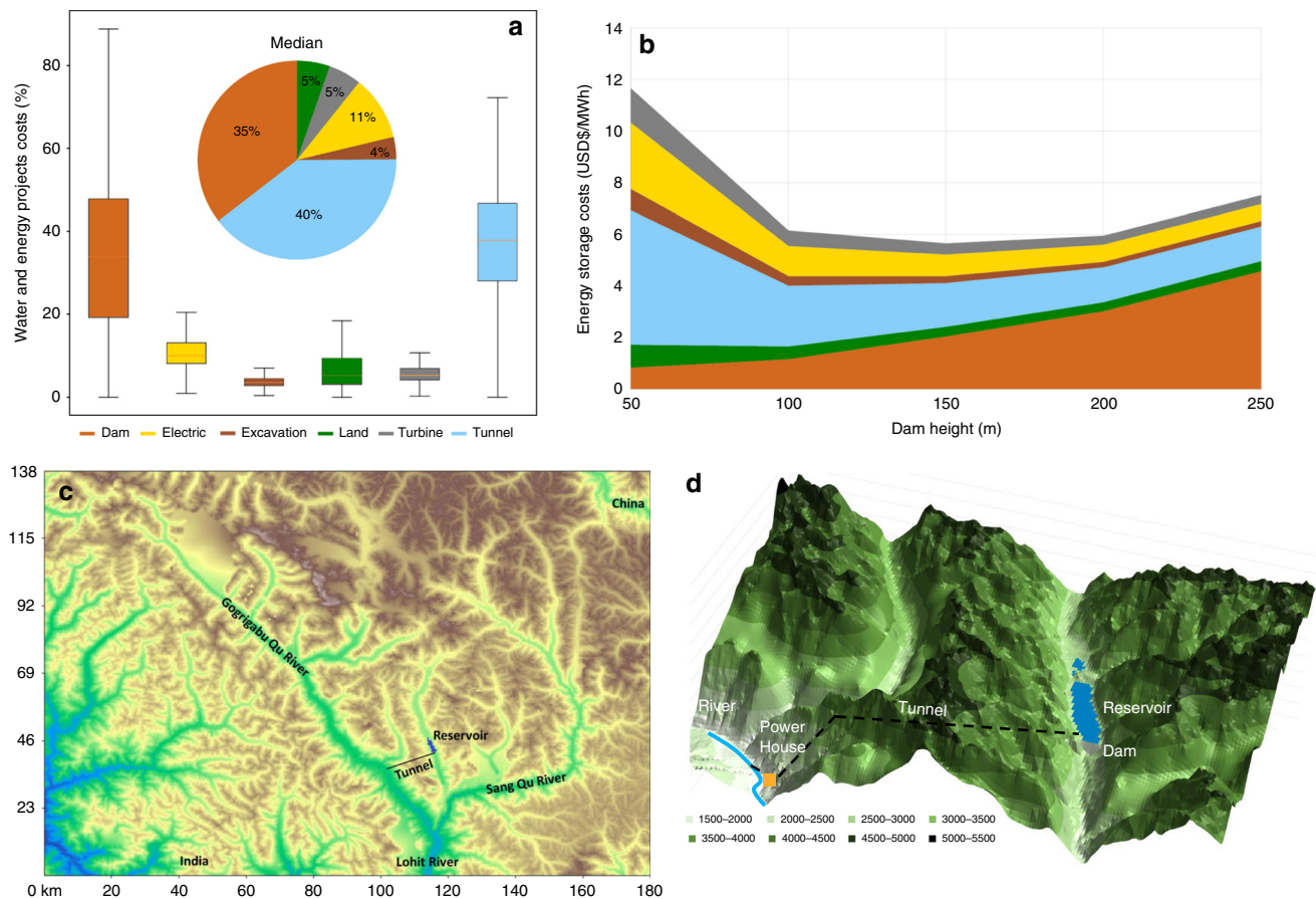
Fig. 1 Seasonal pumped hydropower storage (SPHS) costs and description. a Water and energy SPHS project cost distribution shows that the most expensive components tend to be the tunnel and dam. b Example of energy storage cost variation with cascade according to different heights for the example project in c . The energy storage cost reduces with the increase in dam height due to economies of gains, however, it then increases because the reservoir becomes larger than the amount of water available to be sustainably stored. c Presentation of selected project in Tibet, China, on a topographic map, presenting its tunnel in black and reservoir in purple. d Zoom in the selected project.
