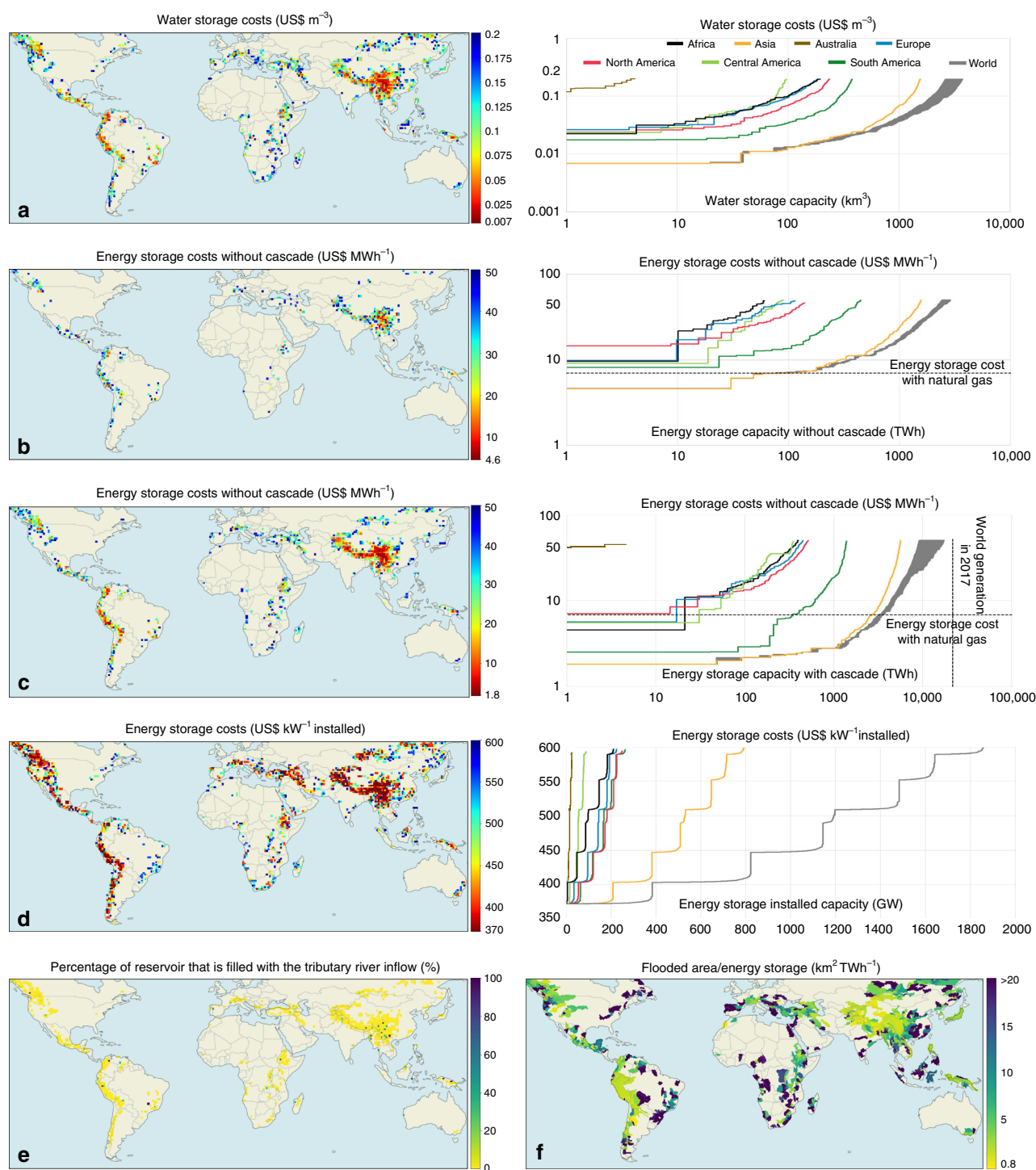
Fig. 2 Seasonal pumped hydropower storage world cost and flooded area maps. a Water storage costs and capacity curve in km 3 . b Energy storage without considering hydropower plants in cascade costs and capacity curve in US$ MWh -1 . c Energy storage considering hydropower plants in cascade costs and capacity curve in US$ MWh -1 . d Additional generation capacity costs and capacity curve in US$ kW -1 . e Percentage of the reservoir that is filled with the river inflow into the SPS reservoir. f Average land requirement for energy storage in different basins.
